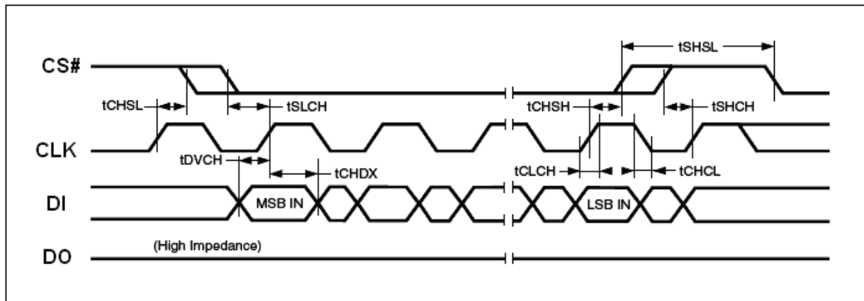
Input Timing
