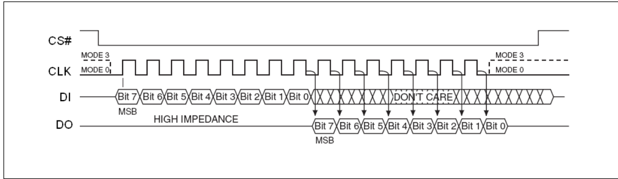
SPI Modes
